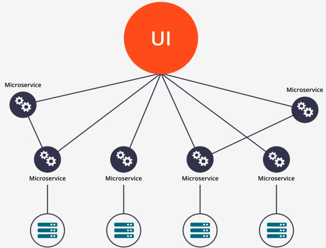
Microservice Architecture
