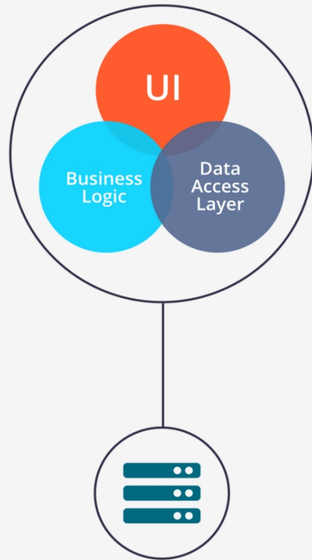
Monolithic Architecture
